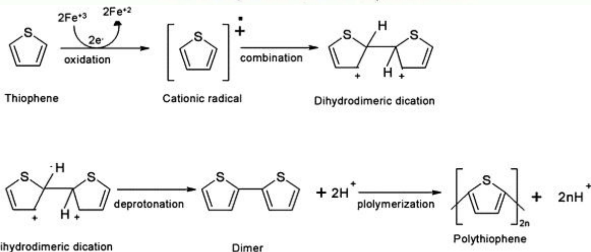
Fig 1.0: Synthesis of Polythiophene (PT)
